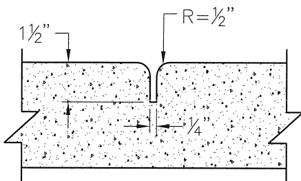
CONTROL JOINT
