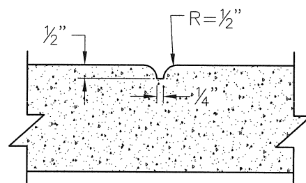
SCORE LINE
